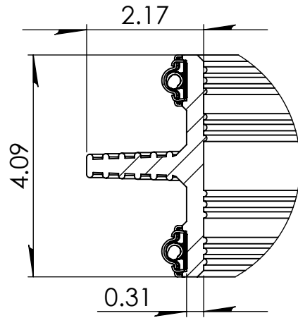
DETAIL C
